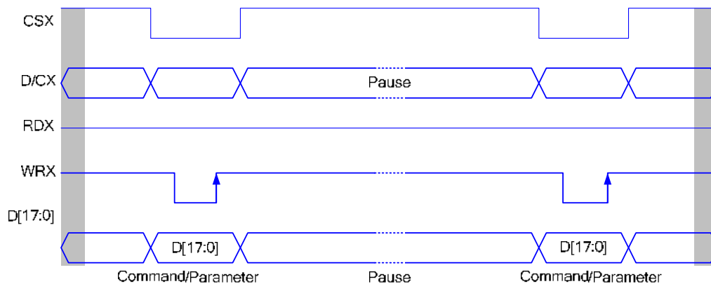
Figure 26 Parallel Bus Pause Protocol (Paused by CSX)
