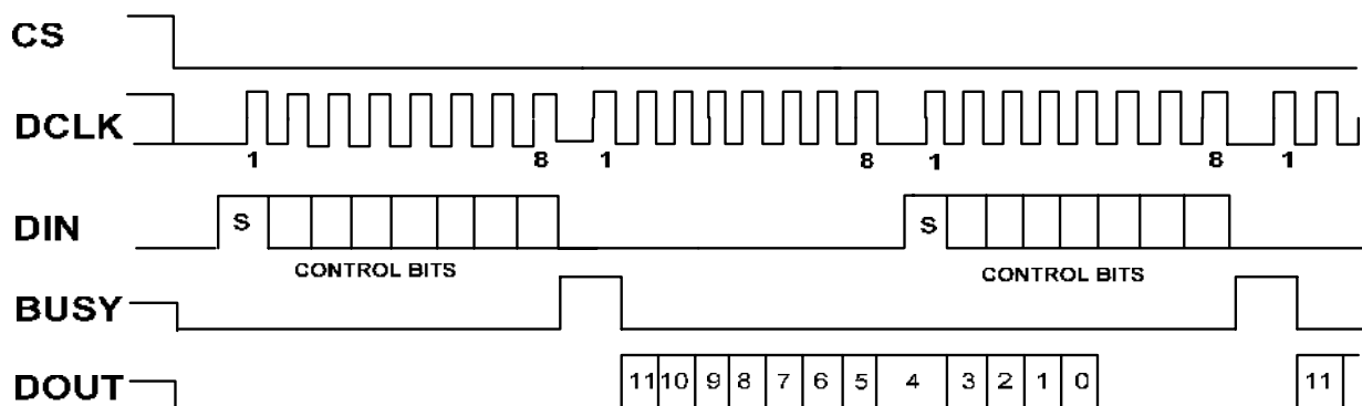
Figure 14. Conversion Timing, 16 Clocks-per-Conversion, 8-Bit Bus Interface.
