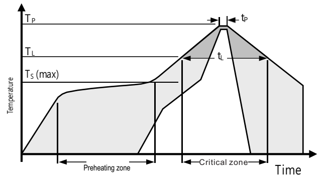
Figure 9 JEDEC Standard welding procedure diagram. T_p \leq 260^\circ\text{C} , t_p < 30 sec, lead-free welding. T_L < 220^\circ\text{C} , t_i < 150 sec, The rate of temperature rise and fall during welding shall be < 5^\circ\text{C}/\text{sec} .
