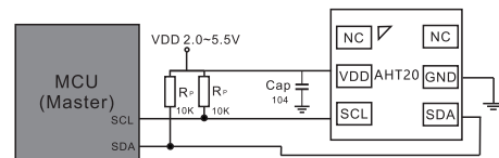
Figure 16 Typical application circuit
