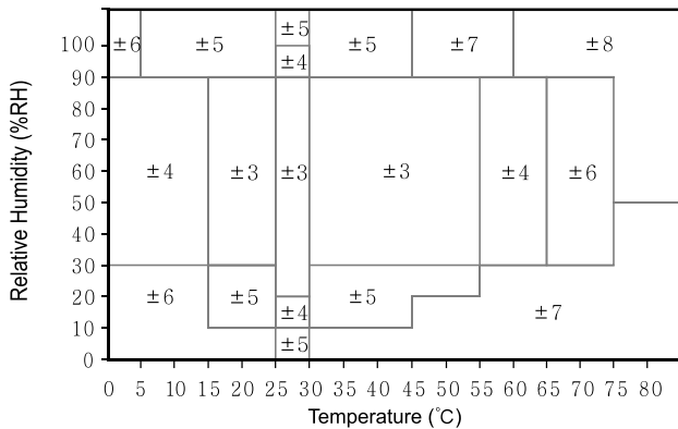
Figure 5 Maximum humidity error between 0~80 °C, unit: (% RH)
