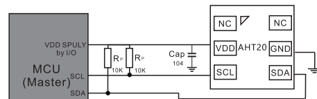
Figure 15-1 Typical application circuit ①, the pull-up voltage and VDD of SCL and SDA are powered by the MCU.
